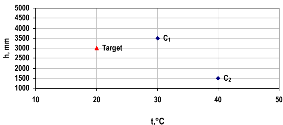
Fig. 2 Coordinate plane
