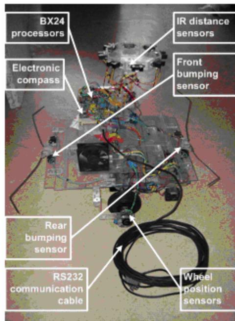
Figure 5. The robotic system.
