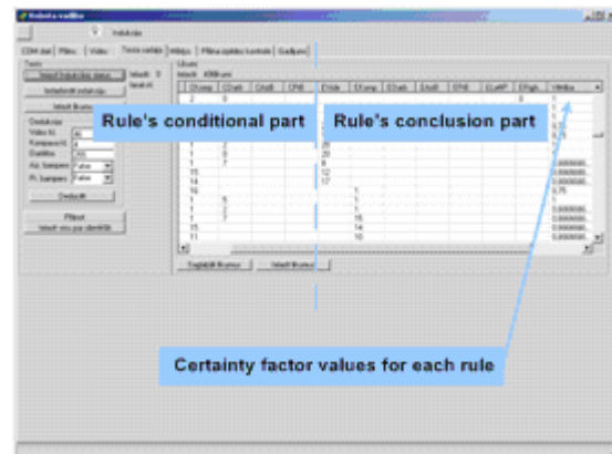
Figure 7. Contr. Software – rule base section.
