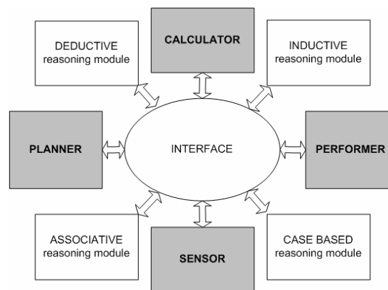
Figure 2. Enhanced architecture
