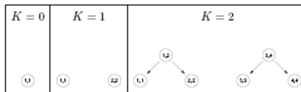
Fig. 1. 2^K -RQP graphs for K \in 0..2
