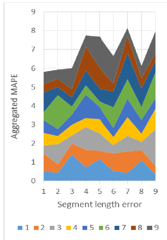
Figure 11.– Dependence between permissible subrules' shifting errors, covered segment error and MAPE
