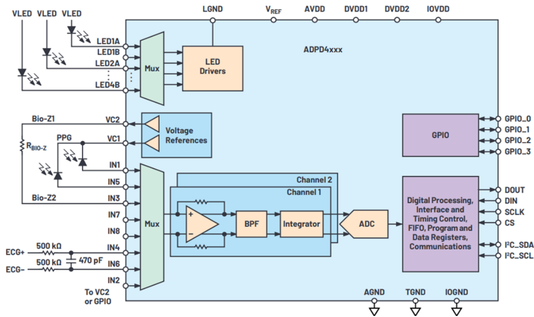
Figure 1. Functional diagram of interface ADPD4xxx for multiparameter sensors
